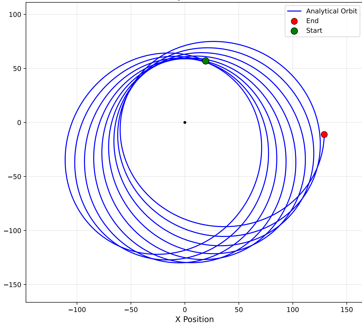
Analytical Orbit
